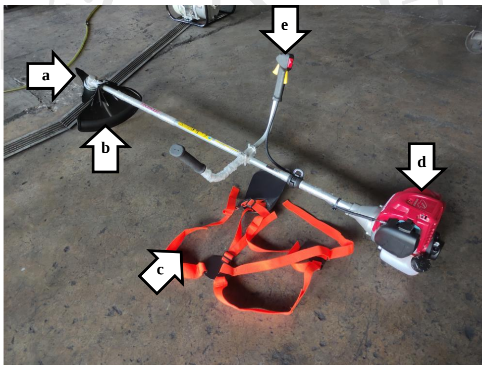
Figure 1. Parts of the HONDA UMK435T Brush Cutter powered by 1.0 kW HONDA GX35 Gasoline Engine include the following: (a) Cutting blade, (b) Safety cover/Deflector, (c) Harness/Strap, (d) Prime mover, and (e) Handle with throttle lever.
